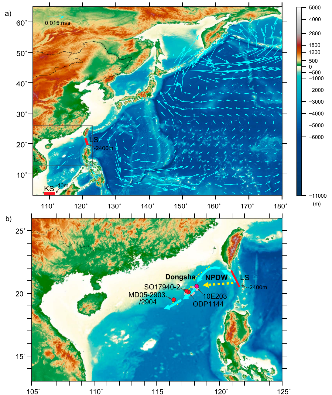
Figure 1. (a) Ocean bathymetry in the North Pacific (color) and ocean currents (m/s) at 1992–2622 m depth at the LGM as simulated in LOVECLIM Earth system model [Menviel et al., 2011]. (b) A schematic map with the enlargement of the black square in Figure 1a to show the topography and current system in the NE part of the SCS, with spatial references of cores locations. NPDW = North Pacific Deep Water. The core 10E203 marked with pink color was the primary core analyzed in this study. The red colored circles are the cores to which we referred. The yellow dashed line is the deep current route proposed by Lüdmann et al. [2005]. The cyan solid line is the deep current path revealed by Liu et al. [2010] and Shao et al. [2007]. Sediment drift: yellow crosses [Shao et al., 2007] and grey shaded area [Lüdmann et al., 2005]. LS and KS represent the Luzon Strait (–2400 m) and Karimata Strait (–40 m), respectively (red bar).
